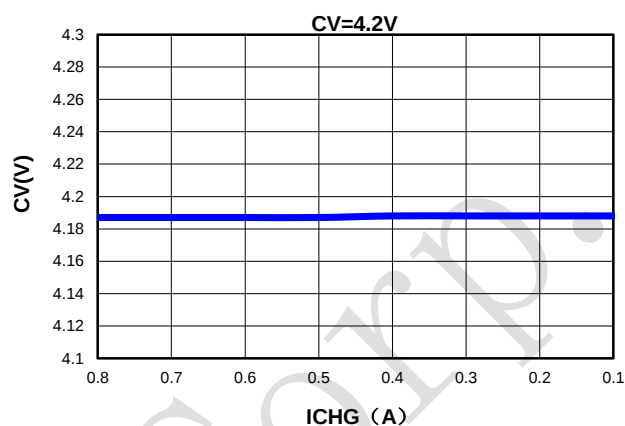
Chart 2 CV vs. ICHG@VIN=5V
