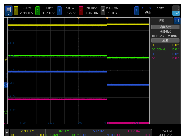
Chart 10 Internal Timer (CC Timer=4hr)
