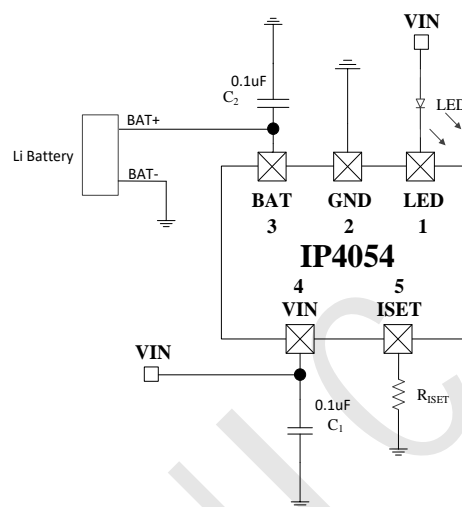
Figure 8 Typical Application Schematic
