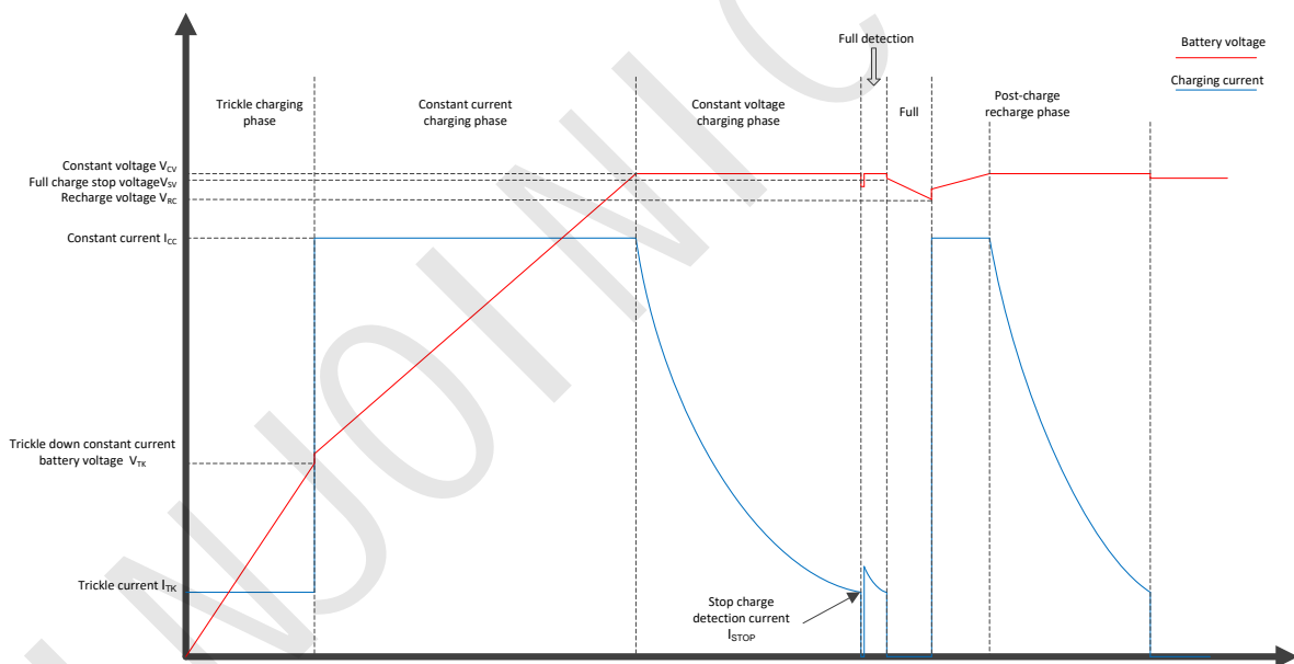
Figure 4 IP4054 Schematic diagram of the charging process
