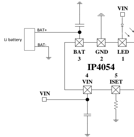
Figure 1 IP4054 Simplified Application Schematic
