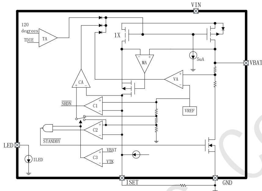
Figure 3 IP4054 Functional Block Diagram
