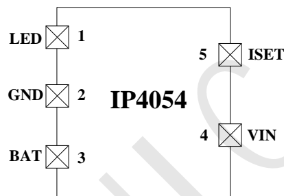
Figure 2 Pin of IP4054
